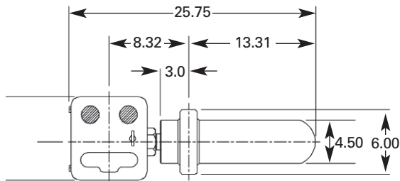
Typical NPT Level Controller & Chamber (Flanged configuration available)
