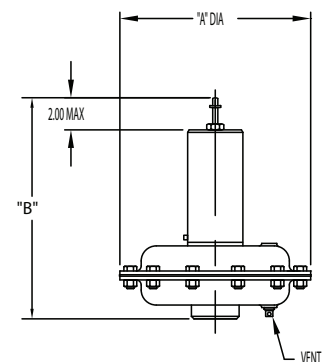
Fig. 15 Direct Actuator Series 2220
