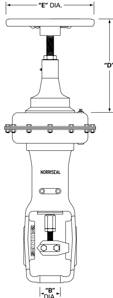
Actuator with Top-Mounted Handwheel
