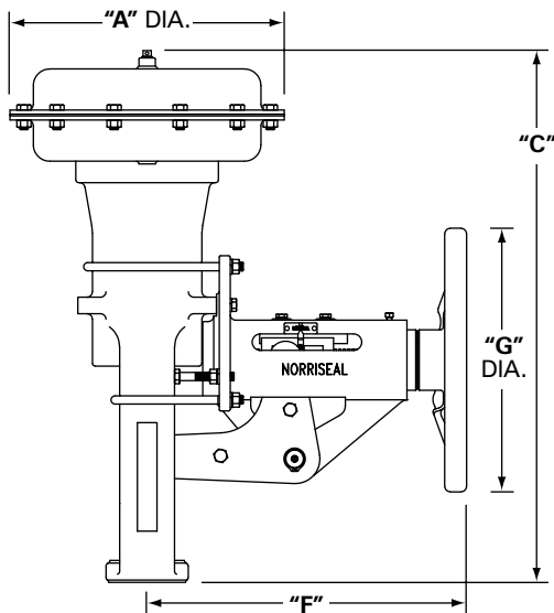
Actuator with Side-Mounted Handwheel
