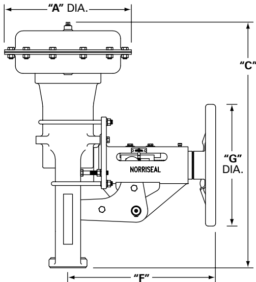
Actuator with Side-Mounted Handwheel
