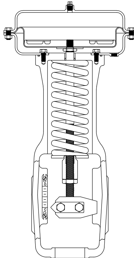
Reverse-Acting (Fail-Closed)
