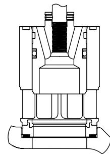
Quick Opening with Soft Insert Flow Down
